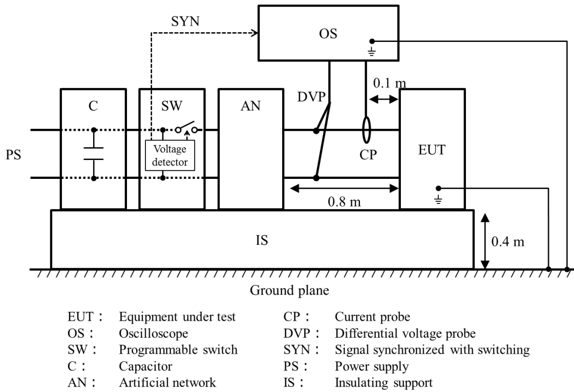
Fig. A.2 Measurement system of transient current
