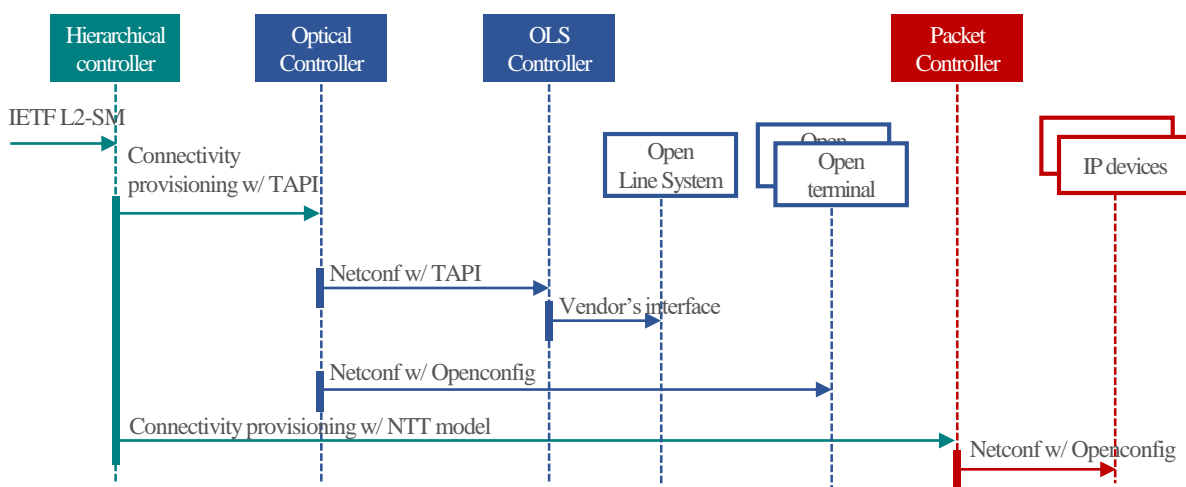
Figure 4. End-to-end provisioning workflow
