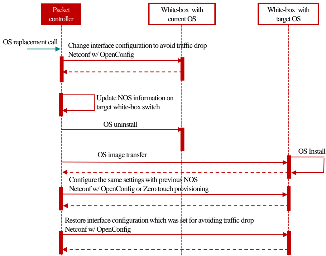
Figure 6. Workflow for automatic NOS replacement procedure
